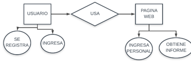
Figure 8. Entity-relationship model.
