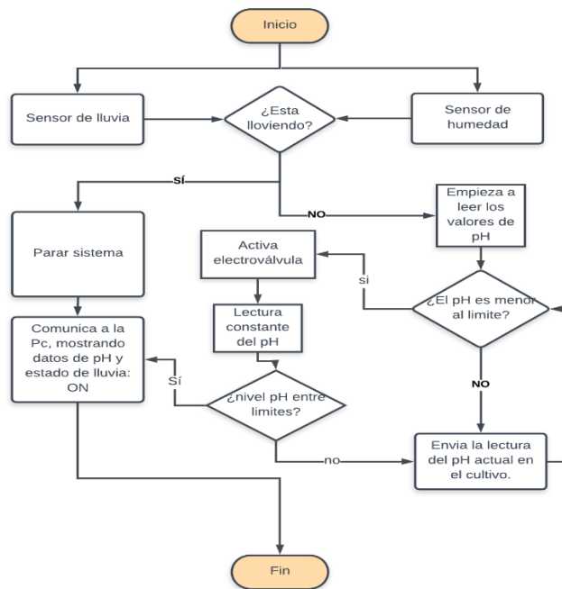
Figure 8. Irrigation diagram.
