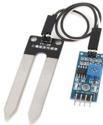
Figure 2. FC-28 module [11].
