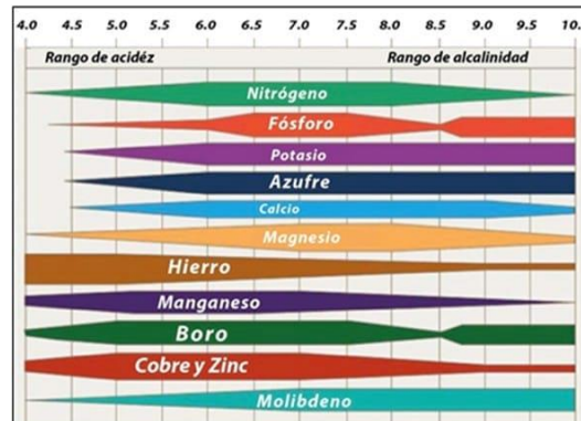
Figure 1. Nutrient availability for soil pH [1].
