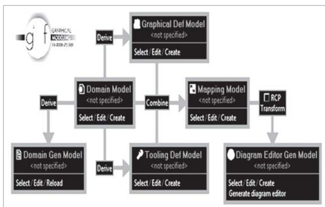
Figura 5. GMF Overview o dashboard. Tomado de T. E. Foundation [17]
